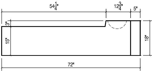
LEFT END VIEW
