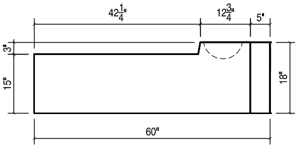
LEFT END VIEW
