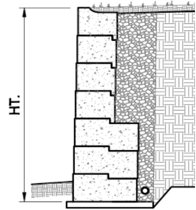
Wall Elevation
